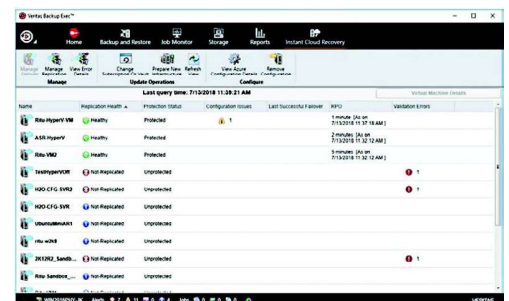
Figure 2. Backup Exec 20.4
